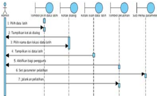
Gambar 9. Rancangan Sequence Diagram Latihan JST
