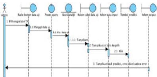
Gambar 10. Sequence Diagram Uji JST
